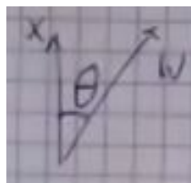
Figure 12.2: Dot product
