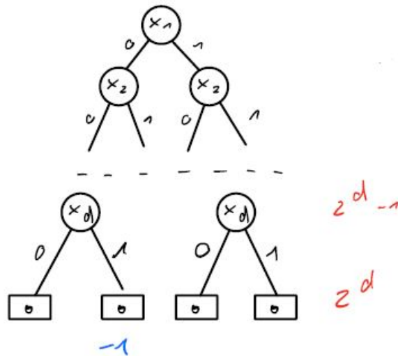
Figure 9.1: Tree building
